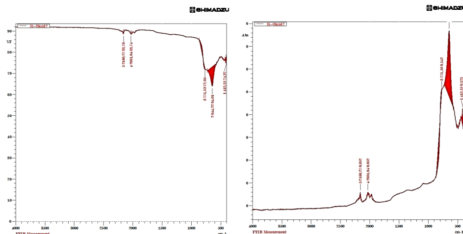
Fig. 2. Smoothing analysis of the transmission and absorption spectrum of \text{SiO}_2/\text{Si}(111)
